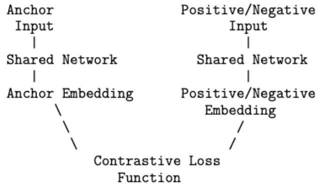
Fig. 6: Siamese network with Contrastive Loss function
